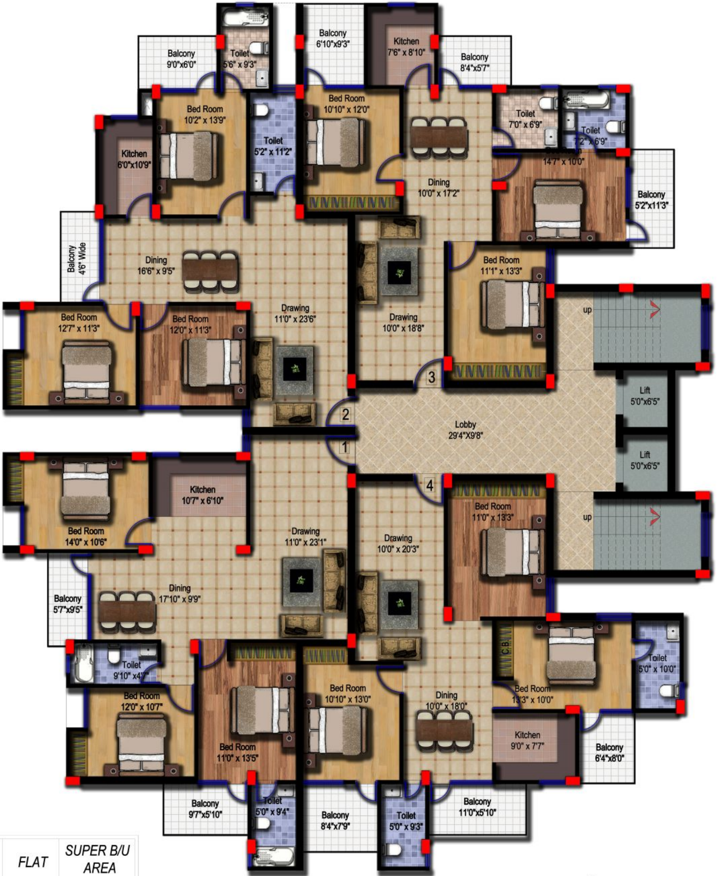
TYPICAL FLOOR PLAN : SECOND TO SIXTH FLOOR
